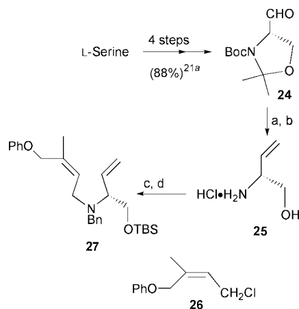
Scheme 6 Reagents and conditions: (TBS = Me 2 t BuSi) (a) Ph 3 P + CH 3 Br − , KHMDS, THF, −78 °C to rt (80%); (b) 6 M HCl (100%); (c) (1) PhCHO, Et 3 N, Na 2 SO 4 , DCM, Δ, (2) NaBH 4 , MeOH, 0 °C, (3) TBSCl, imidazole, DMF (70%); (d) 26 , K 2 CO 3 , cat. NaI, MeCN (86%).
